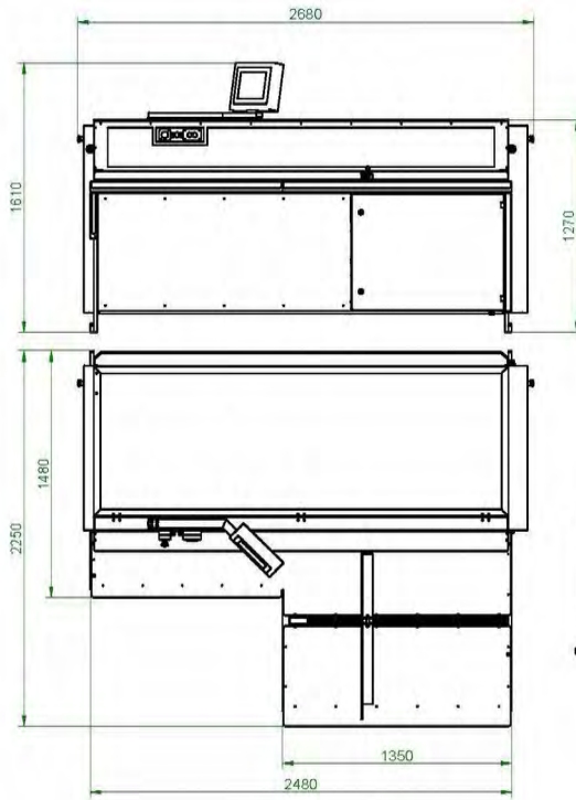
ECOMATIC 23DC, ECOMATIC 23DC plus - floorplan
